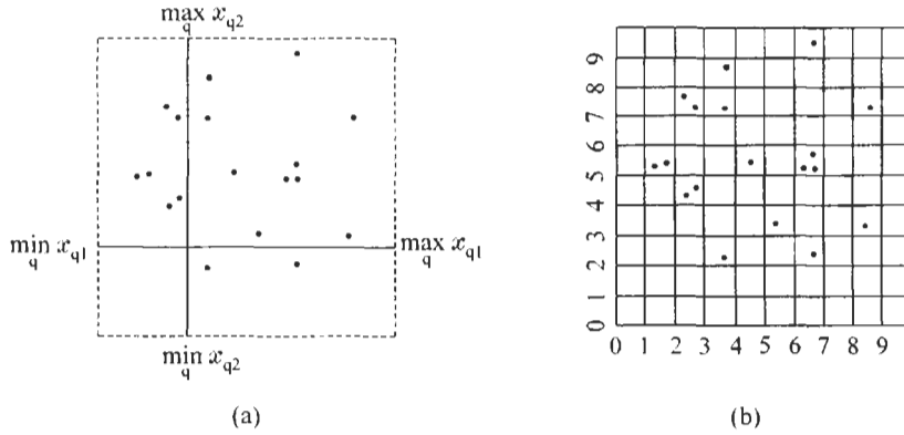
FIGURE 15.10: (a) The original data set X . (b) Normalization of the data set X in [0, r - 1]^l , with r = 10 , and discretization. The nonempty hypercubes define the discrete binary set.
