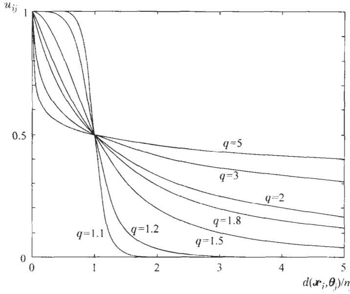
FIGURE 14.16: Plots of the membership function for various values of q .
