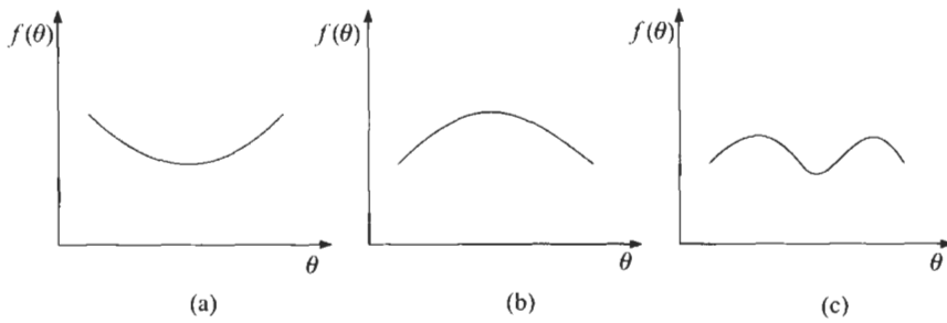
FIGURE C.5: (a) A convex function, (b) a concave function, and (c) a function that is neither convex nor concave.
