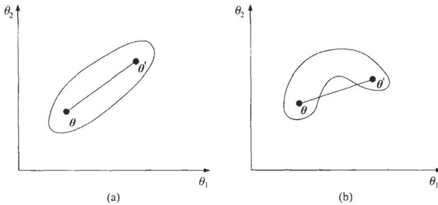
FIGURE C.6: (a) A convex set and (b) a nonconvex set of points.
