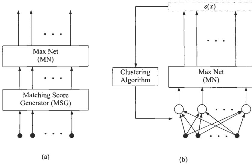
FIGURE 12.4: (a) The neural architecture. (b) Implementation of the BSAS algorithm when each cluster is represented by its mean vector and the Euclidean distance between two vectors is used.
