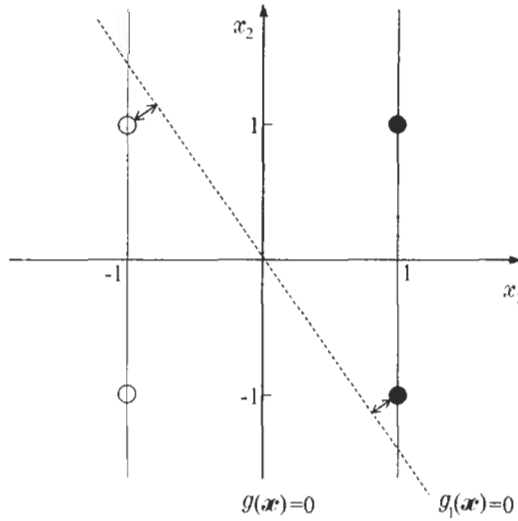
FIGURE 3.10: In this example all four points are support vectors. The margin associated with g_1(x) = 0 is smaller compared to the margin defined by the optimal g(x) = 0 .
