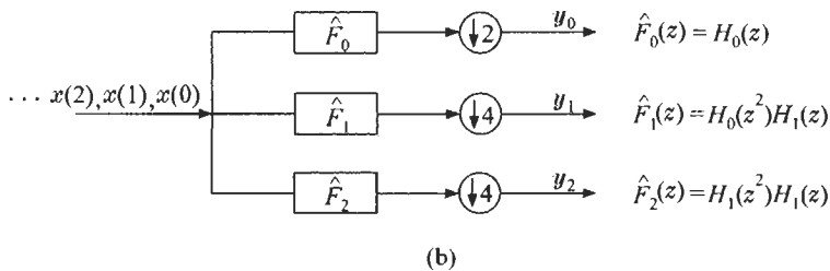
FIGURE 6.6: (a) Noble identity I and (b) equivalent filter bank of Figure 6.5.
