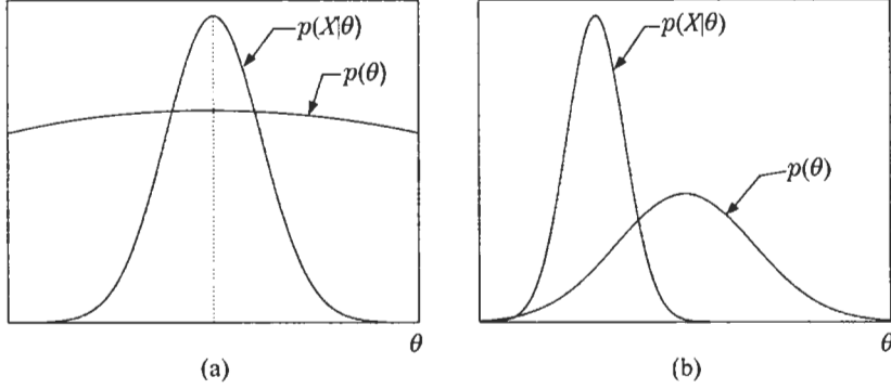
FIGURE 2.7: ML and MAP estimates of \theta will be approximately the same in (a) and different in (b).
