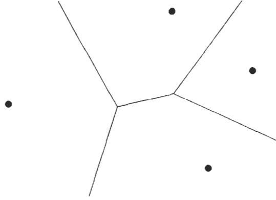
FIGURE 2.11: An example of Voronoi tessellation in the two-dimensional space and for Euclidean distance.
