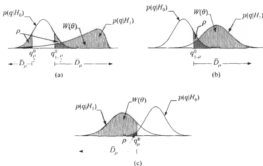
FIGURE 16.1: Critical regions of (a) a two-tailed test, (b) a right-tailed test, and (c) a left-tailed test. q_a^0 is the a percentile of q under H_0 . 1
