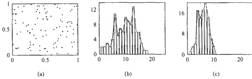
FIGURE 16.10: (a) The data set X . (b) The distribution of the distances of the point [0.5045, 0.4764]^T from the remaining points in X . (c) The distribution of the distances of the point [0.0159, 0.8089]^T from the remaining points in X .
