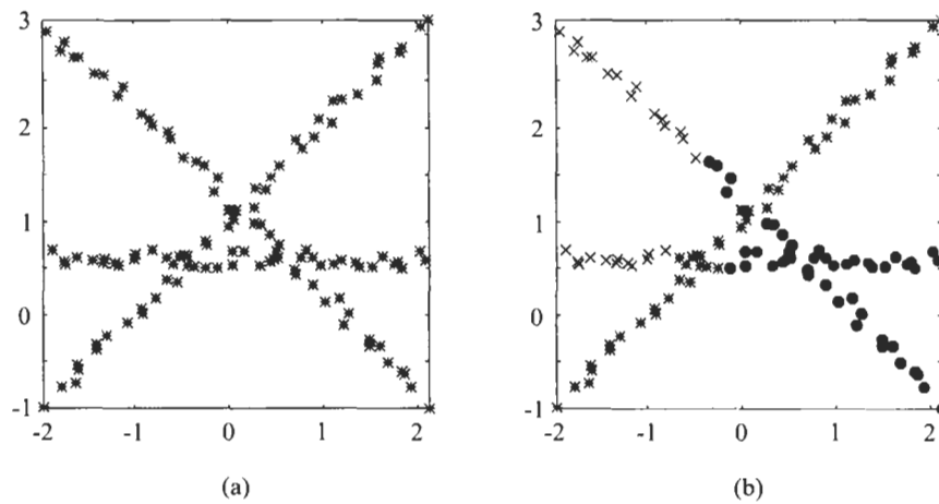
FIGURE 14.14: (a) The data set X for Example 14.10(b). (b) The results of the G-K algorithm.
