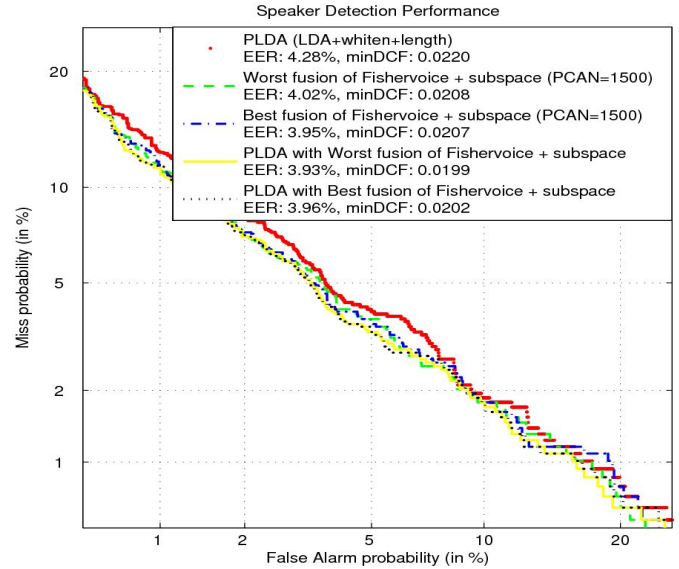
Figure 2: Fusion results with other systems on NIST SRE08 male tel-tel task (projection matrix trained with full set)
