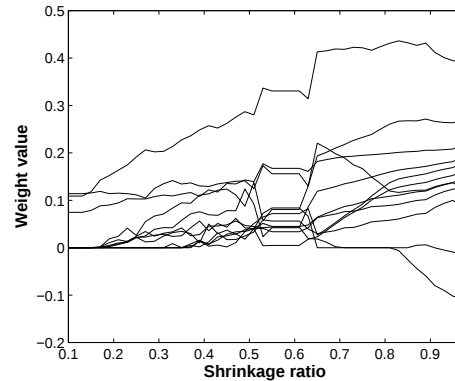
Figure 2: Weight evolution of the Elastic-net regularization, with \alpha = 0.7 , as a function of normalized t .
