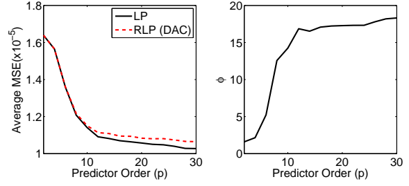
Figure 1: Effect of prediction order on prediction error and penalty function (the use of the DAC sequence in regularization is explained in subsection 2.4).
