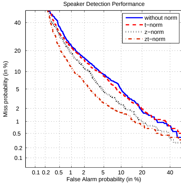
Figure 1: DET curves for various types of score normalization using large numbers of imposters. Core condition of the NIST 2006 SRE, English language trials only.
