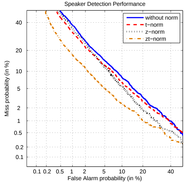
Figure 2: DET curves for various types of score normalization using large numbers of imposters. Core condition of the NIST 2006 SRE, all trials.
