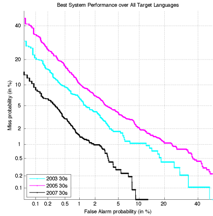
Figure 1: Best system performance on 30 second closed set general language recognition trials in the 2003, 2005, and 2007 evaluations
