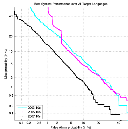
Figure 2: Best system performance on 10 second closed set general language recognition trials in the 2003, 2005, and 2007 evaluations
