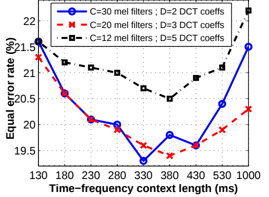
Figure 3: Effect of the time-frequency context size.
