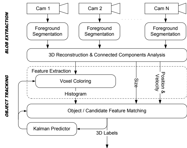
Figure 2. The system block diagram showing the chain of functional modules
