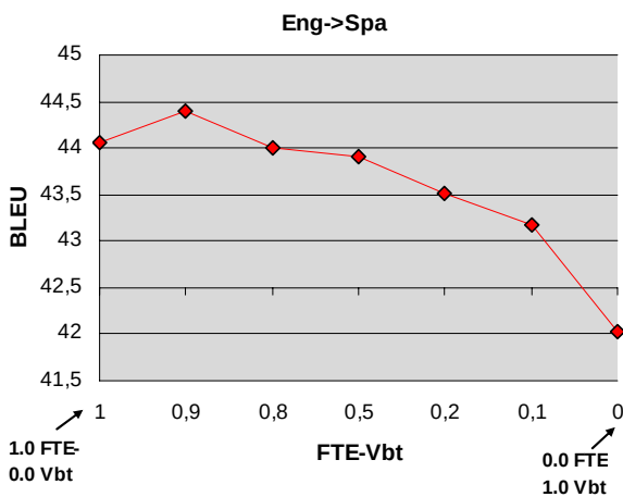
Figure 2. Results of Eng to Spa translation (dev).
