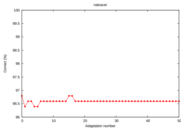
Figure 4. Sentence accuracy rate in each iterative adaptation for nalcacer speaker.
