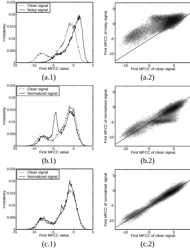
Figure 2. Scattergrams and histograms between the first MFCC in non-silence frames for different signals. The line in the scattergrams represents the function x = y .
