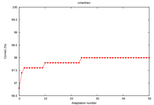
Figure 2. Sentence accuracy rate in each iterative adaptation for cmartinez speaker.
