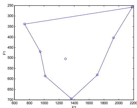
Figure 1: Formants of the Catalan vowels
