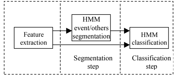
Figure 3. CMU acoustic event detection system
