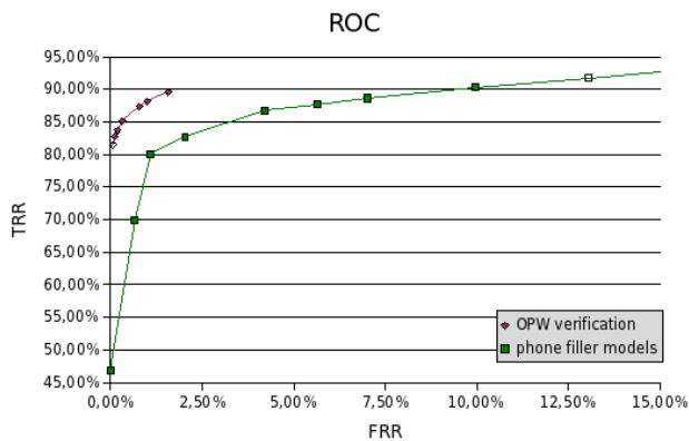
Figura 1. TRR vs. FRR
