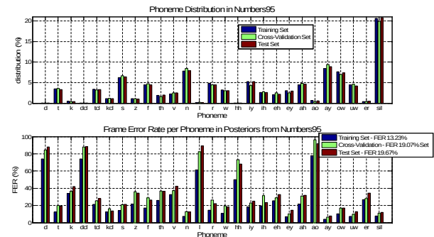
Figure 2. Analysis in Posterior sets: a) Phoneme Distribution and b) Frame Error Rate per Phoneme in a posteriori probabilities .
