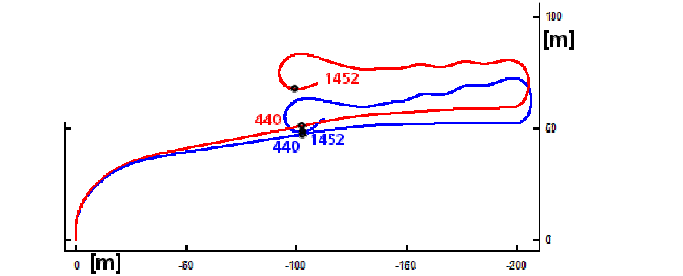
Figure 11: “Real life” test run and path reconstruction using uncalibrated yaw rate (red) and calibrated yaw rate (blue). Frame 440 and frame 1452 are the frames where the true trajectory intersects itself.
