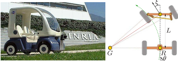
Fig. 5. The Cycab vehicle and its kinematics.
