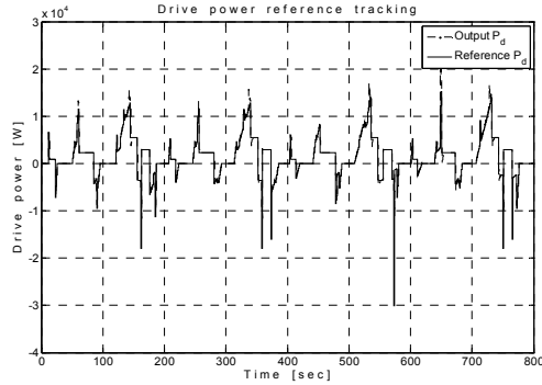
Fig. 10. Drive power reference tracking
