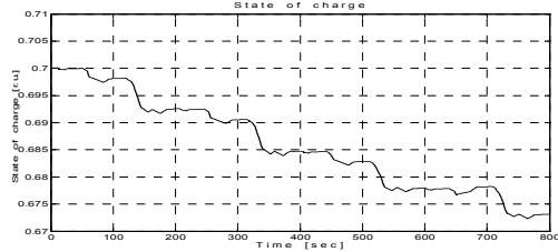
Fig. 11. State of Charge
