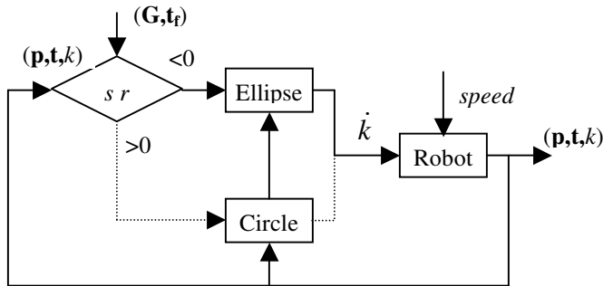
Fig. 4. Robot control loop
