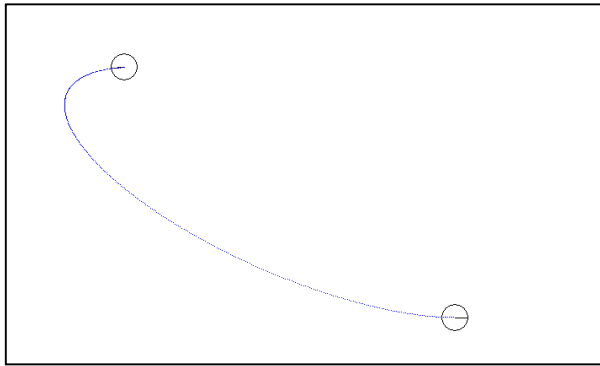
Fig. 5. Elliptical trajectory
