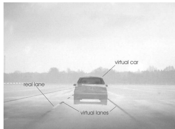
Fig. 6: Augmented reality demonstration of the Vehicle in the Loop
