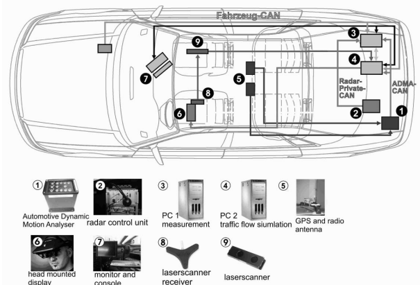
Fig. 4: System architecture of the Vehicle in the Loop
