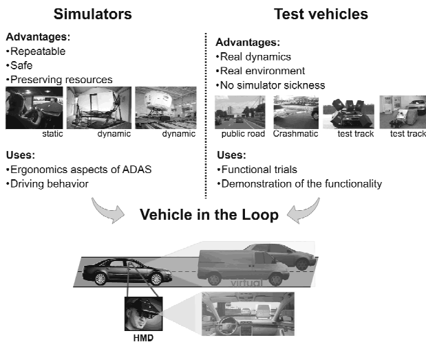
Fig. 2: Vehicle in the Loop – Linking a simulator and a test vehicle
