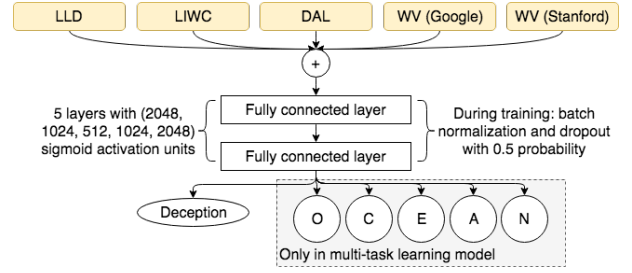
Figure 2: Diagram of multi-task learning MLP model (variant ii).
