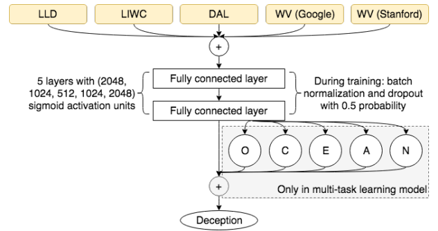
Figure 2: Diagram of multi-task learning MLP model (variant ii).
