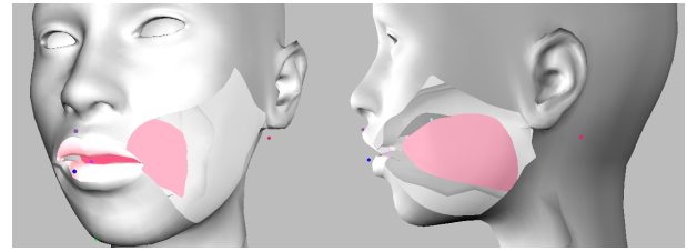
Figure 2: Example visualization
