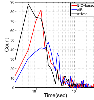
Figure 2: The length distributions of target speaker segments. The average length for BIC-based, aIB and s-ivec diarization are 446, 567 and 326 seconds, respectively.
