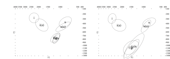
Figure 8: 2-sigma Ellipses for the vocalic elements in Taiyuan rising diphthongs in male (left) and female (right) speakers.
