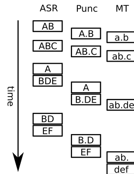
Figure 1: Update Protocol
