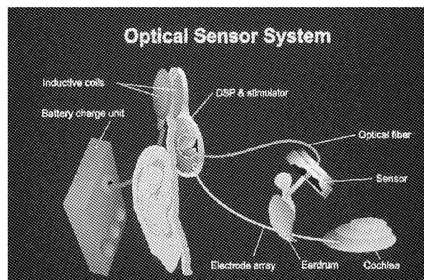
Figure 9: The overall concept of a totally implantable cochlear implant with the sensor placed in the middle ear, and all the electronics and the rechargeable battery in the mastoid process.
