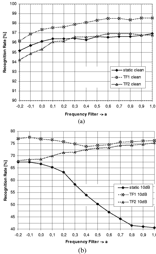
Figure 3: Recognition rate in terms of the FF and TF used in the parameterization for (a) clean and (b) white noise speech with SNR=10dB
