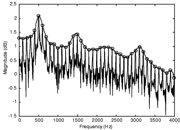
Fig. 2. Speech spectrum with SEEVOC peaks (circles) and SEEVOC envelope (using cubic spline interpolation).
