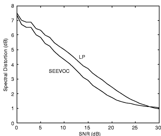
Fig. 6. Comparison of spectral distortions obtained from LP analysis and SEEVOC (true pitch TP = 100 Hz).
