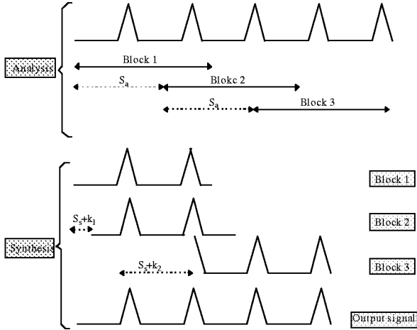
Figure 2: PSOLA method
