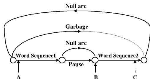
Figure 1: Word sequence model (basic model).
