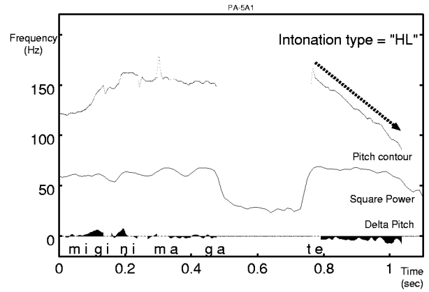
Figure 4. Falling intonation
