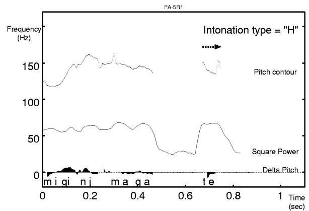
Figure 6. Neutral intonation
