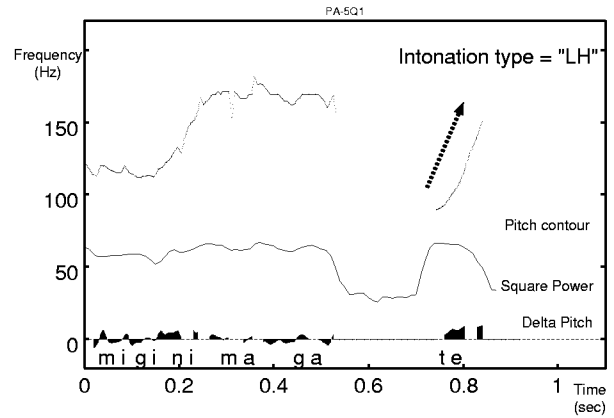
Figure 5. Rising intonation
