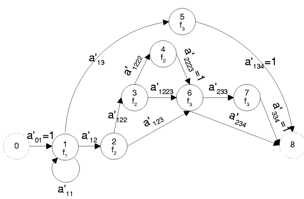
Figure 4: The first order equivalent of the HMM illustrated in Figure 2.
