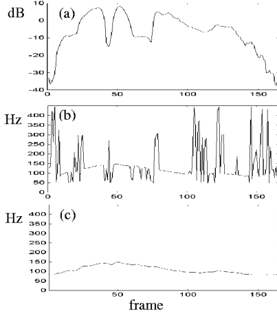
Figure 7: Referring to the the Italian noisy voiced word /lavan'daja/ ('washerwoman'): in plot (a) the frame-by-frame signal to noise ratio corresponding to a global 0dB SNR is indicated; in (b) the pitch estimate from the original Summary Correlagram [2] is given, while in (c) the final estimated pitch computed with the proposed algorithm is illustrated.
