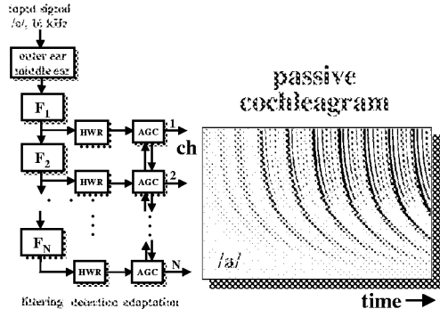
Figure 1: Outline of the Lyon's cochlear model. The passive cochleagram refers to the Italian vowel /a/.
