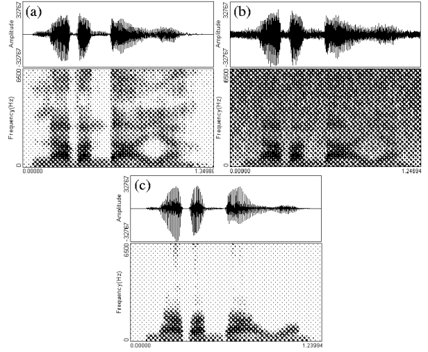
Figure 8: Application of the 'correlagram subtraction' enhancement technique to the Italian noisy (0dB SNR) word /lavanda'ja/ ('washerwoman'): (a) clean [SOUND 1053_01.wav], (b) noisy [SOUND 1053_02.wav] and (c) enhanced [SOUND 1053_03.wav].
