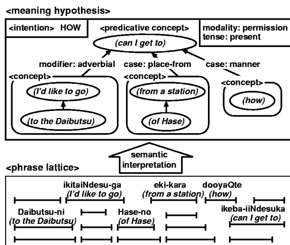
Figure 1: Concept-driven semantic interpretation.
