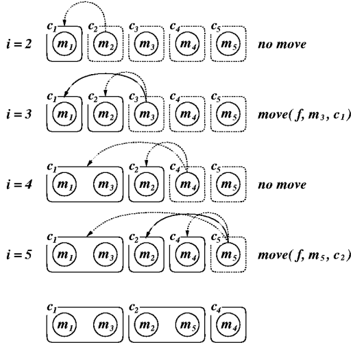
Figure 1: Clustering algorithm.
