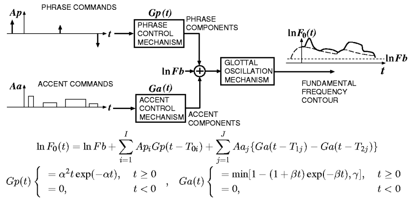
Figure 1: A command-response model for F_0 contour generation.
