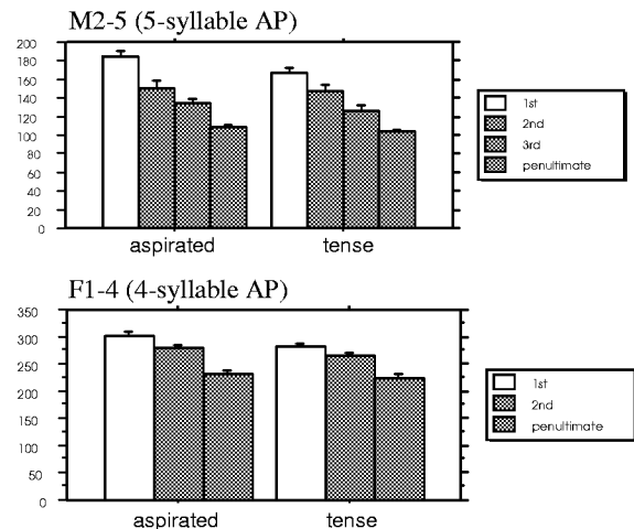
Figure 5: F0 value of the vowel with an aspirated or tense onset in each syllable position in an AP.
