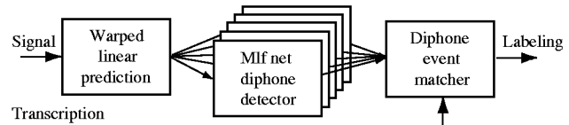
Figure 1: Block diagram of the automated labeling system.
