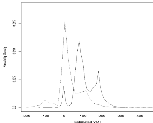
Figure 5: Distributions of VOTs for “r” (dotted) and “d” (solid). Obtained by running the second pass VOT extraction algorithm on a first pass that corresponds to a forced alignment of the HMM models with the true identity.
