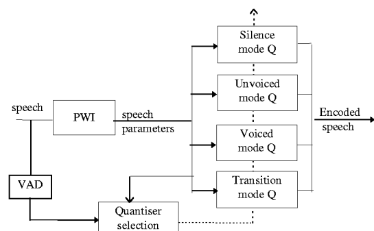
Figure 1 : Scheme of the source control variable bit rate PWI encoder
