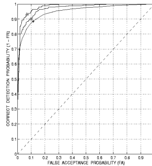
Fig. 3. ROC curves for detection of "loud" speech from neutral using pitch (input vector lengths: * = 1; o = 5; \Delta = 10)
