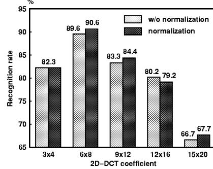
Figure 2: Effect of intensity normalization. (DCT coefficients)
