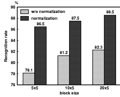
Figure 1: Effect of intensity normalization. (subsampling)
