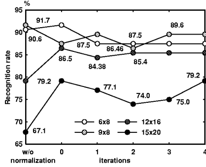
Figure 4: Effect of location-normalized training. (DCT coefficients)
