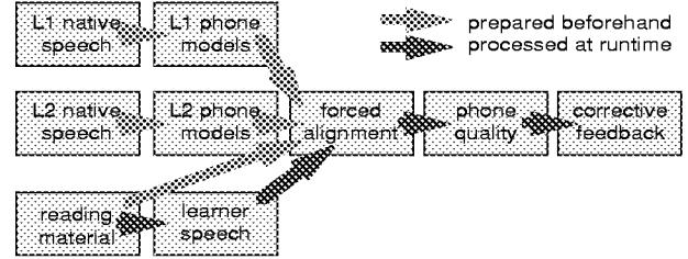
Figure 1: Process flow of bilingual phone recognizer. L1 and L2 HMMs are separately on native speech but combined during recognition. The learner receives categorical articulatory advice on phone quality.
