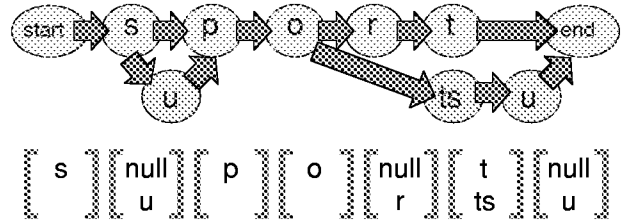
Figure 2: Phone network for the English word "sport" showing possible pronunciation errors by Japanese learners. Above: insertion, substitution and deletion of phones are shown as alternative paths branching off the main path. Below: phone lattice corresponding to the network. Insertions and deletions are represented by null phones.
