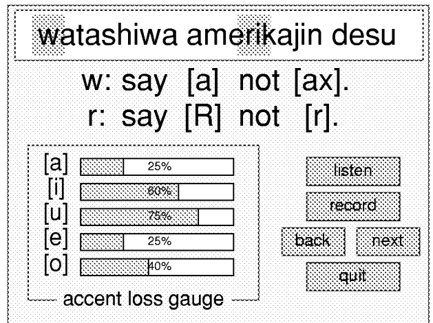
Figure 3: Graphical user interface (GUI) of phone-quality system. The learner receives categorical articulatory advice on phone quality for each mispronounced phone, and an "accent loss gauge" indicating allophone reduction ratios. For explanation purposes, the figure is in English and shows only vowels. The GUI is written in Tcl/Tk.
