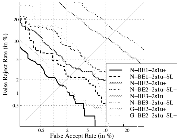
Figure 1: DET-curves [6] based on same-sex impostor attempts for the Nuance verifier 2 (N) and the GIVES/lrmm system (G) with LPCC-based features. Experiments are the three first BEs modified to have 2s1u enrollment (a '+' in the legend indicates a modified BE enrollment set). For all cases a DET-curve for the subset with same-language impostor tests have been included (SL).
