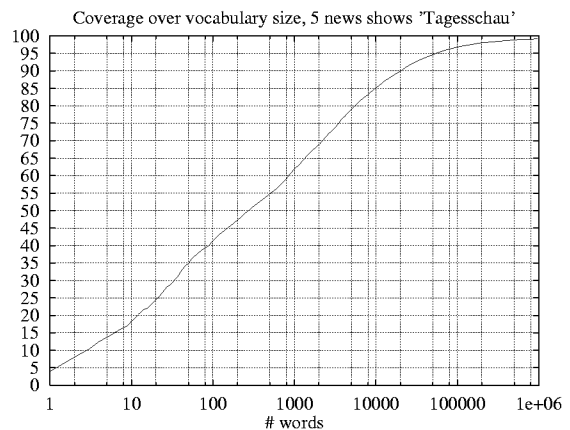
Figure 1. Coverage over vocabulary size for the test set
