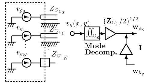
Figure 3: Equivalent circuit and signal flow for source.
