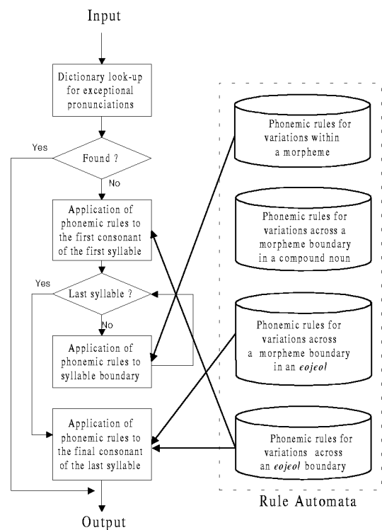
Figure 2: An obligatory phonemic rule processing module for a noun, adverb or adnoun input.
