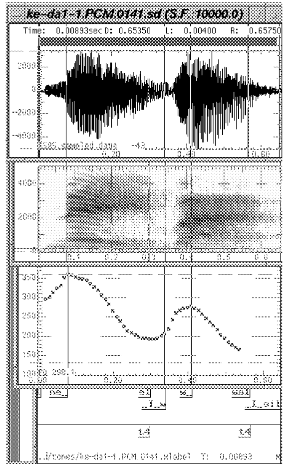
Figure 4. An example of segmentation based on the proposed syllabic structure, where “eI” and “waI” are the nuclei of the respective syllables. Each of F0 contours of the nuclei keeps the basic form of the fourth tone(falling tone).
