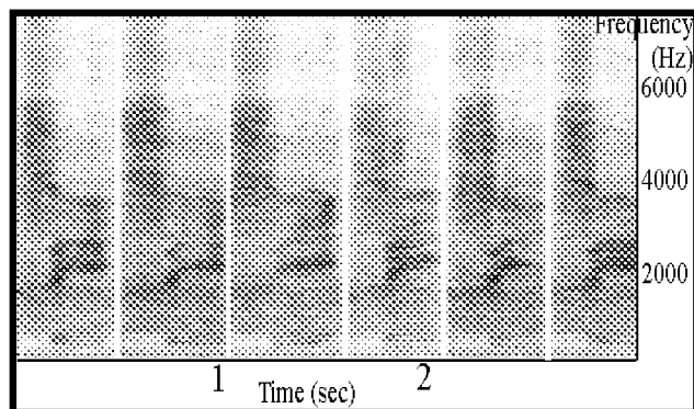
Figure 1: Spectrogram of the six different tonal phonemes /si/.
