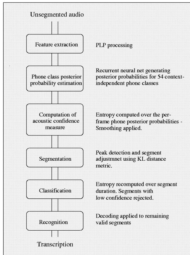
Figure 3: A summary of the segmentation system.
