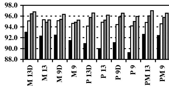
Figure 1: Word-level accuracy results for each of the 10 features using the four initial grammar and duration-limit combinations. The horizontal axis codes are explained in Section 4.1 The black bar is for the SIL grammar and 2SD limits, the white bar is for the GAR grammar and 2SD limits, the dark-gray bar is for the SIL grammar and the 5P limits, and the light-gray bar is for the GAR grammar and the 5P limits.
