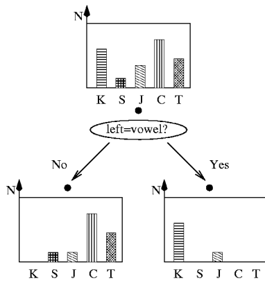
Figure 2: Language distribution of tree node
