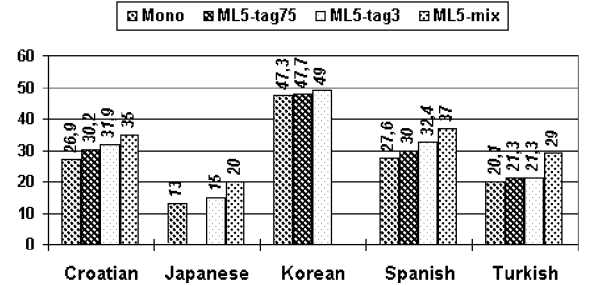
Figure 4: Results for multilingual setup [Error Rate]
