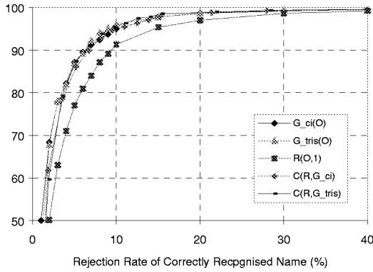
Figure 4: UV performance on OOV name strings at vocabulary size of 40.
