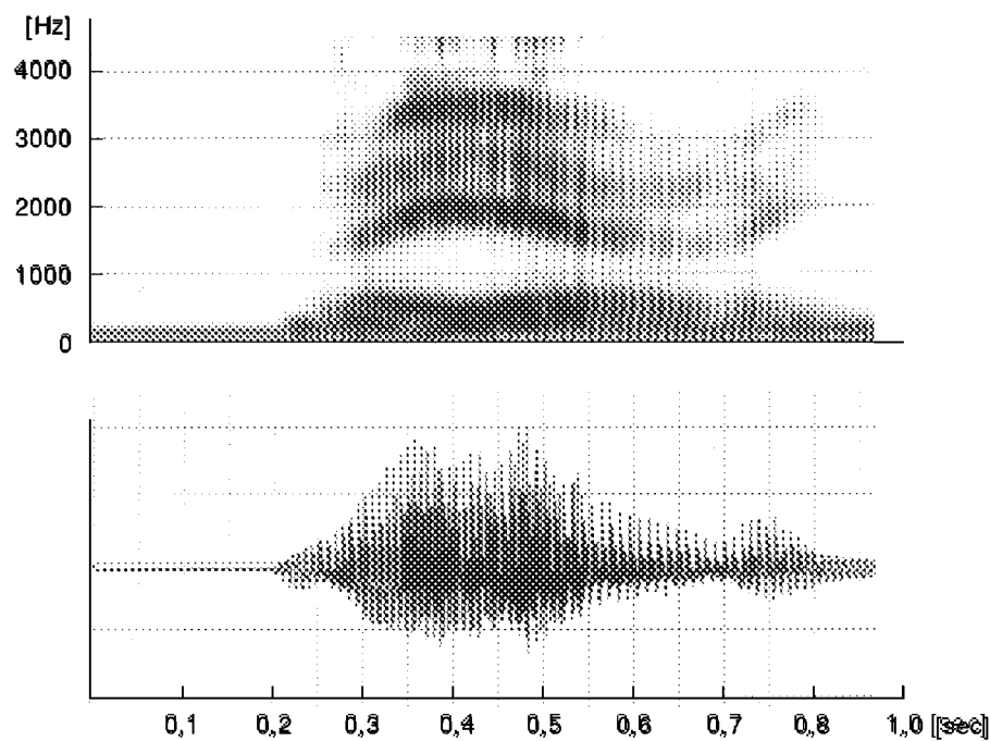
Figure 2: Spectrogram, above, and waveform, below, of voiced velar approximant/fricative pronunciation of /r/ in the Norwegian word "rir" (= (he) rides), [ʁi:ʁ]. Male speaker.
