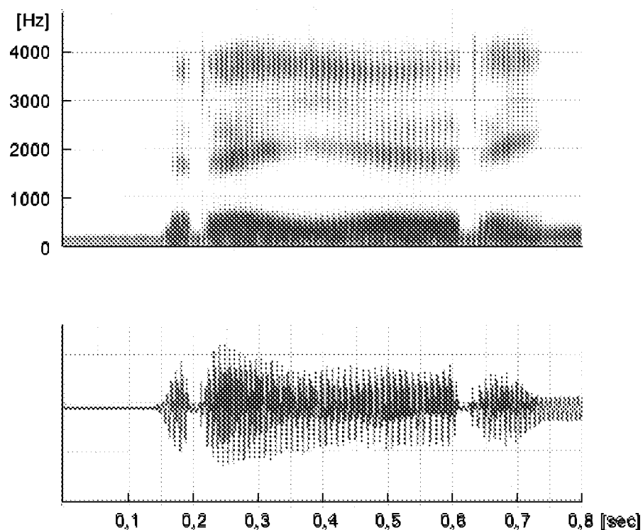
Figure 1: Spectrogram, above, and waveform, below, of voiced apical tap pronunciation of /r/ in the Norwegian word "rir" (= (he) rides), [ʁi:ʁ]. Male speaker.
