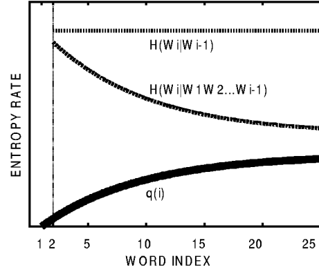
Figure 2: Global shape of the entropy of bigram language model H_M(W_i|W_{i-1}) , true conditional entropy H(W_i|W_1W_2 \cdots W_{i-1}) and the insertion penalty function q_{\text{opt}}(i) .
