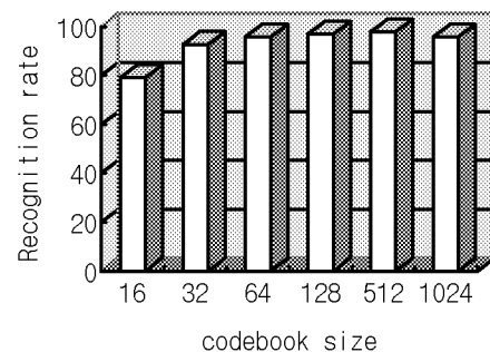
Figure 1 The VQ model performance test results vary according to codebook size
