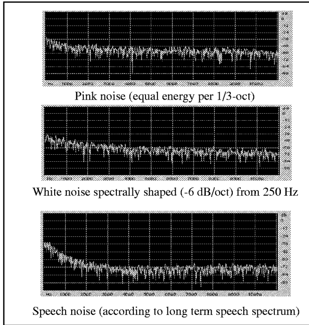
Figure 1: Noises used in the experiments. In the following sections the noise will be referred to pinkvl , pinkilt and speech from, respectively top to bottom in this figure. These noises have been extracted from the NATO RSG 10 database [12].
